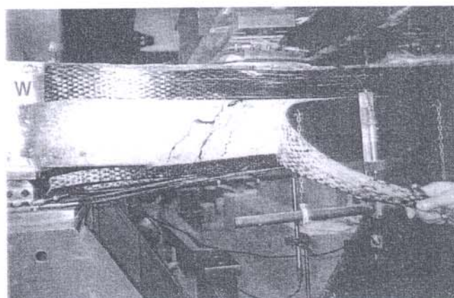
Fig. 9—Specimen Wall2 after failure.
