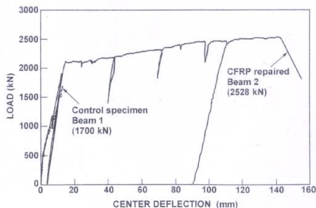
Fig. 16—Load-deflection behavior of beam specimens.
