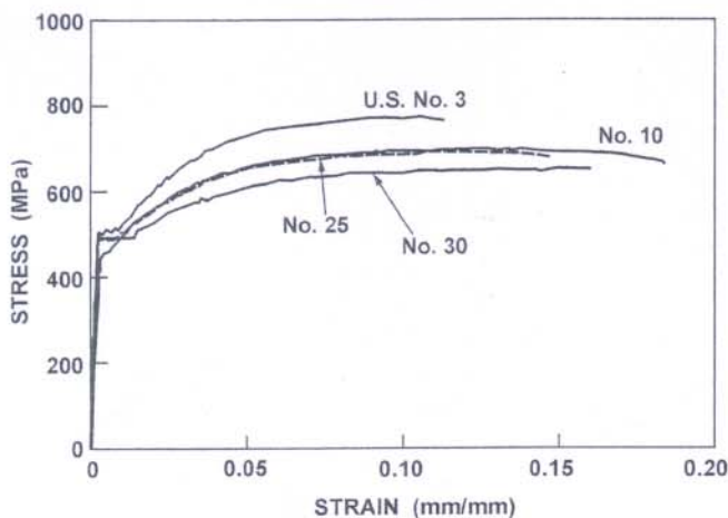
Fig. 4—Tensile stress-strain characteristics of steel.
