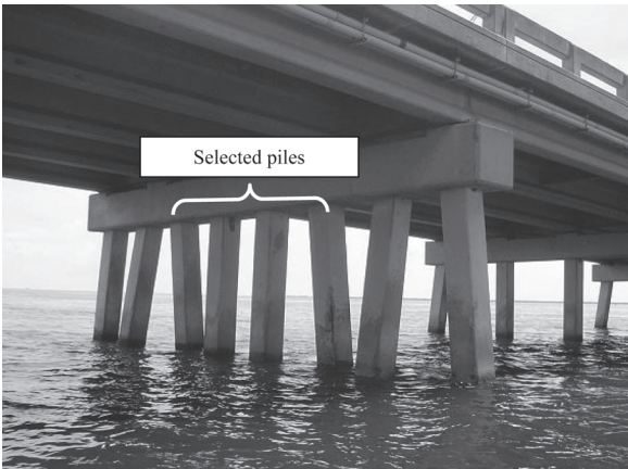
Figure 9 — Selected Piles, Gandy Bridge, Tampa
