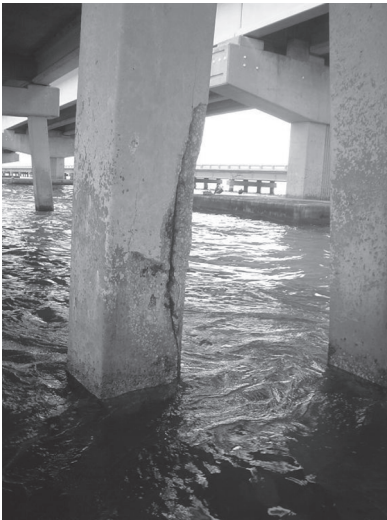
Figure 8 — Heavily Corroded Pile, Gandy Bridge, Tampa
