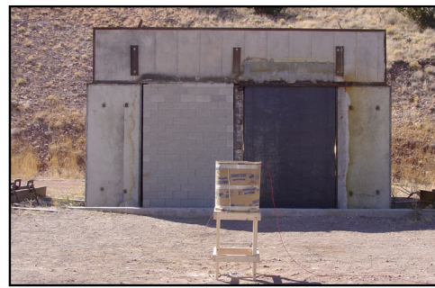
Figure 2: URM wall test specimens ready for blast test
